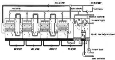
Multi-Effect Distillation (MED)
